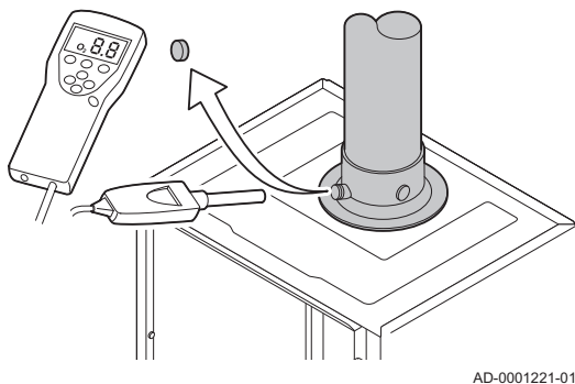
Afb.62 Rookgasmeetpunt
