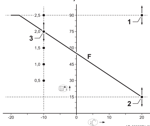
Afb.49 Interne stooklijn
